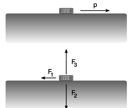
h / A coin slides across a table. Even for motion in one dimension, some of the forces may not lie along the line of the motion.
